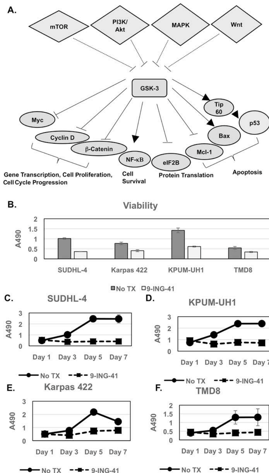
Figure 1: Viability and proliferation of lymphoma cells with 9-ING-41 treatment. (A) Schematic representing GSK-3 up-stream regulators and down-stream targets and their role in cellular processes in cells. It should be noted that several of the target proteins are misregulated in cancer cells. Only target proteins relevant for this paper are shown for simplicity. (B-F) 10,000 cells (SUDHL-4, KPUM-UH1, Karpas 422, TMD8) per 96-well plate well were left untreated or treated with 1 \mu M 9-ING-41 in triplicate, and the number of cells on days 1, 3, 5 and 7 were calculated using the MTS assay. Briefly, 20 \mu L of MTS reagent was added to cells and incubated for 2 hours and, the absorbance at 490 nm (A490) was read using a Biotek plate reader. Error bars represent std. deviation between replicates. Day 3 viability is shown in B.
